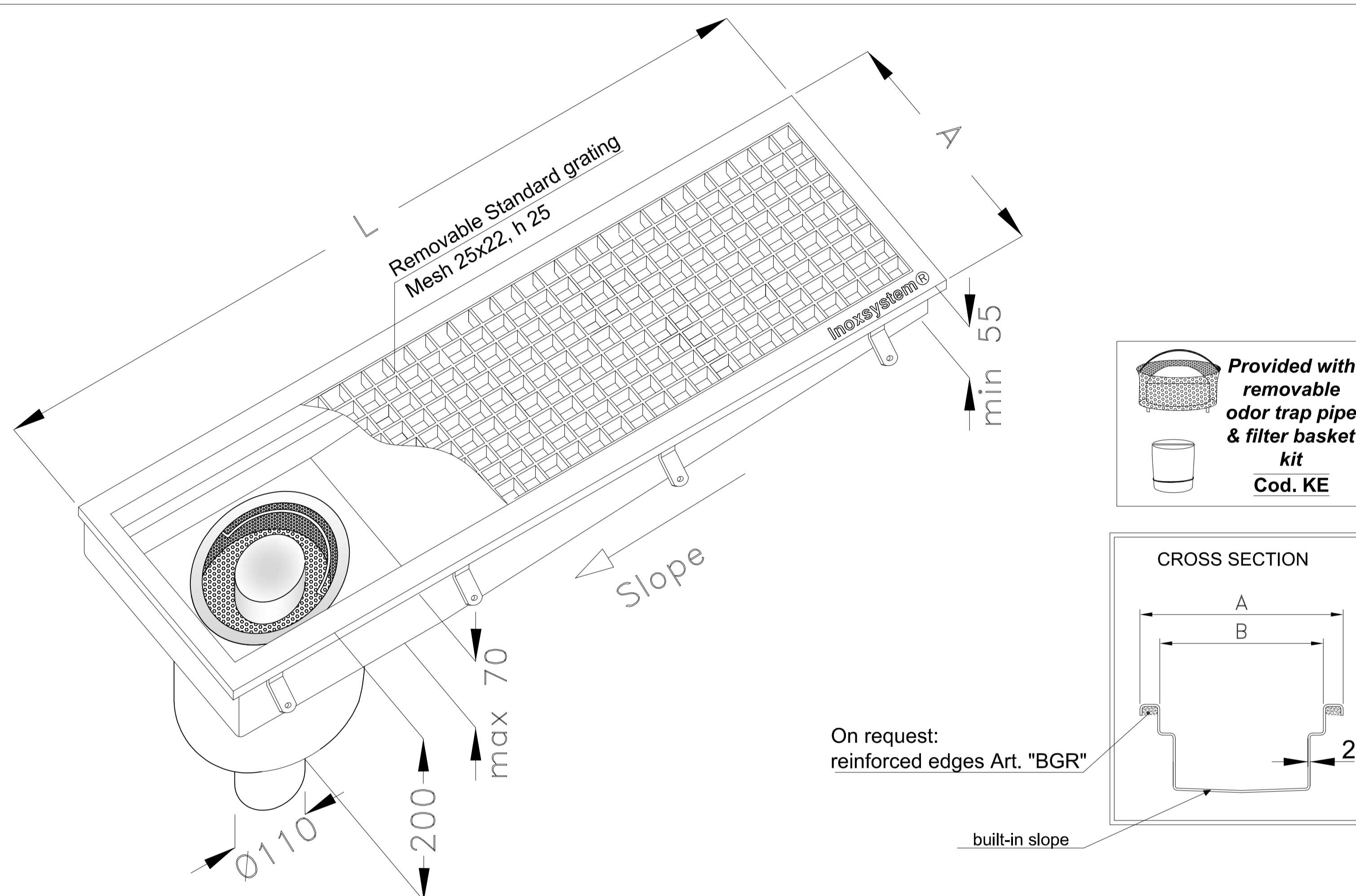
Grade 304 stainless steel (grade 316 on request) - Sheet thk. 2 mm
