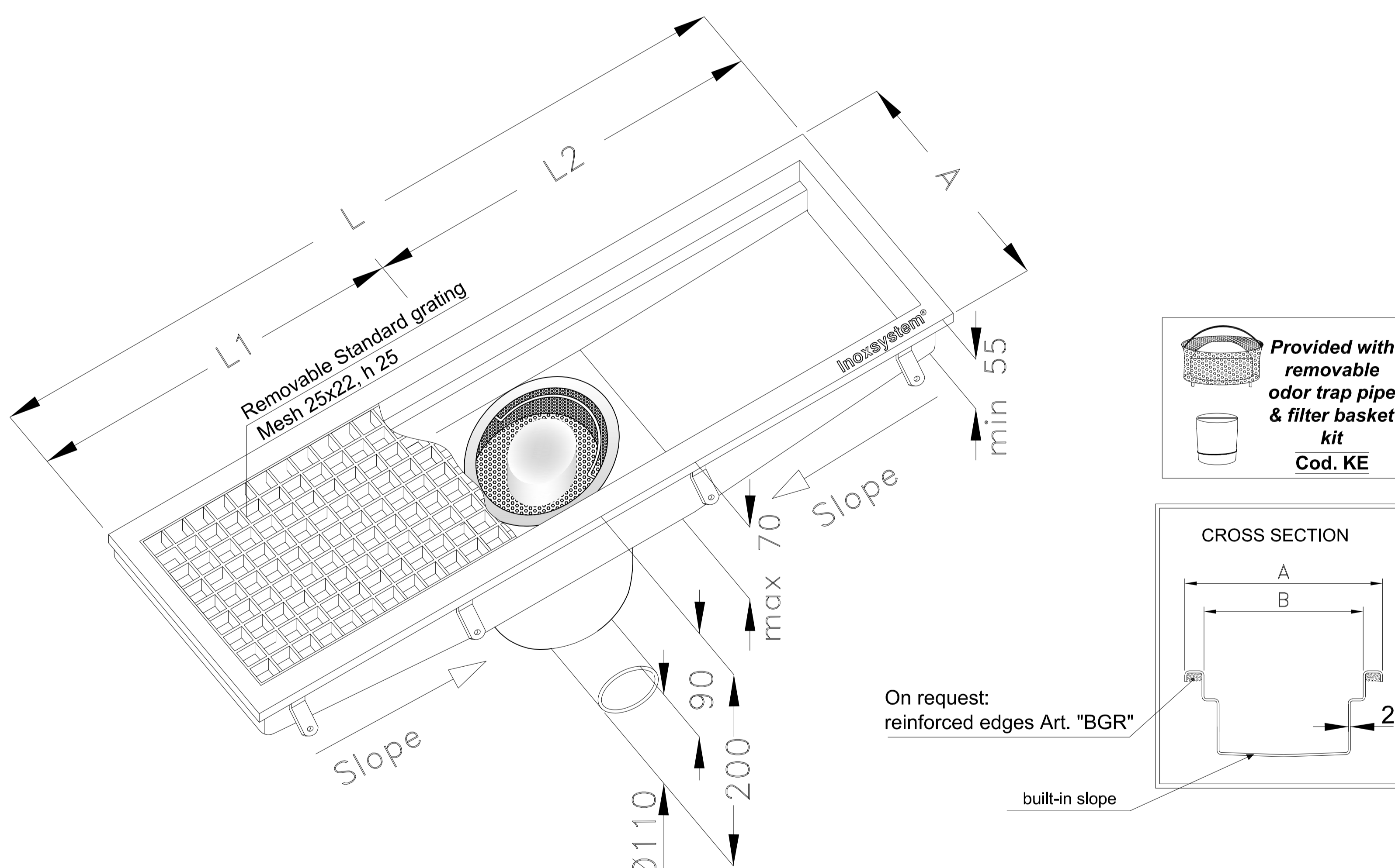
Grade 304 stainless steel (grade 316 on request) - Sheet thk. 2 mm
