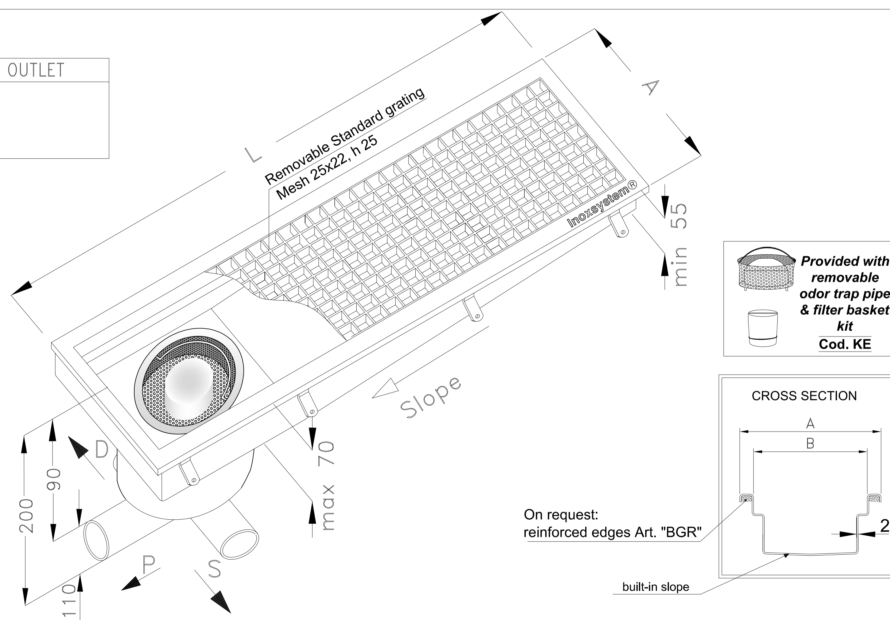
Grade 304 stainless steel (grade 316 on request) - Sheet thk. 2 mm
