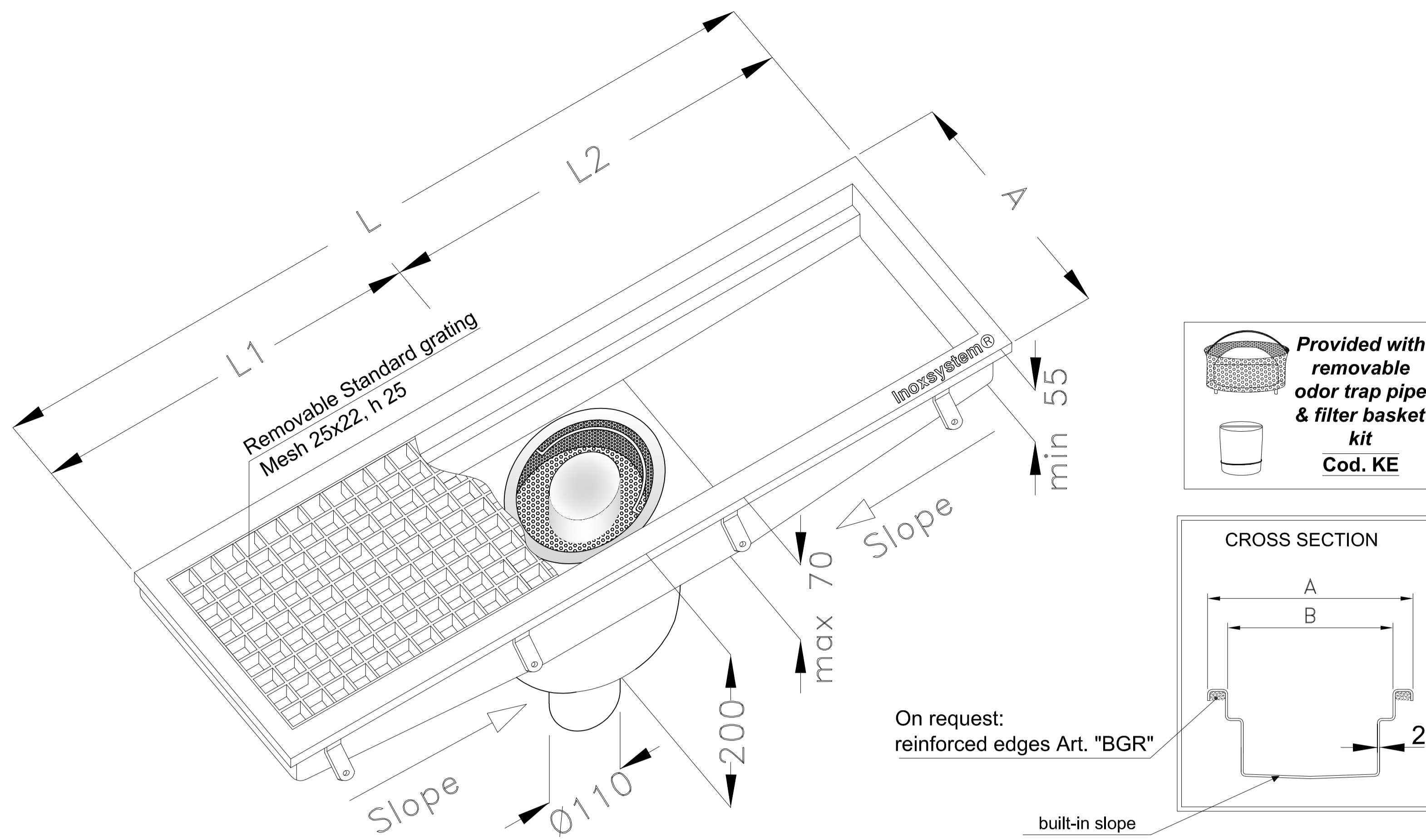
Grade 304 stainless steel (grade 316 on request) - Sheet thk. 2 mm
